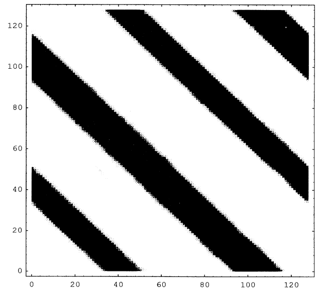
FIG. 2. Average site density of stopped cars in model A ( 128 \times 128 streets) in the jammed phase, for a car density n = 0.7 and a randomness \gamma = 0.1 . Different values are represented by different gray levels ranging from black (site always empty) to white (site always occupied). This illustrates the multistrip structure of the jammed phase in model A.
